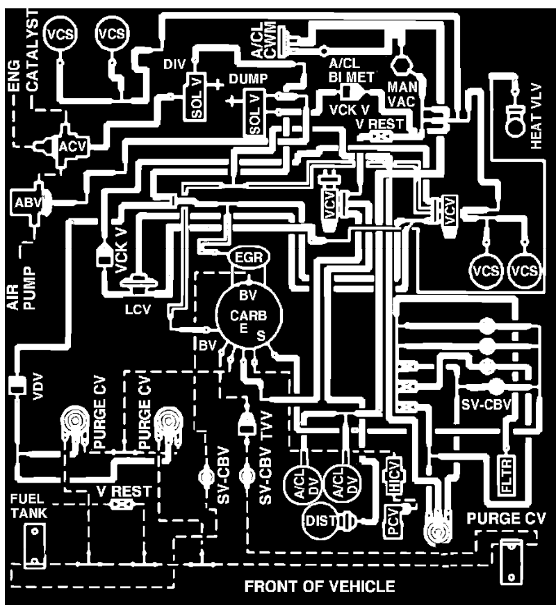
Fig. 23 Vacuum hose routing. 1985 V8-302 H.O. w/4 Bbl. & man. trans. calib. code 5-21A-R01 Federal
